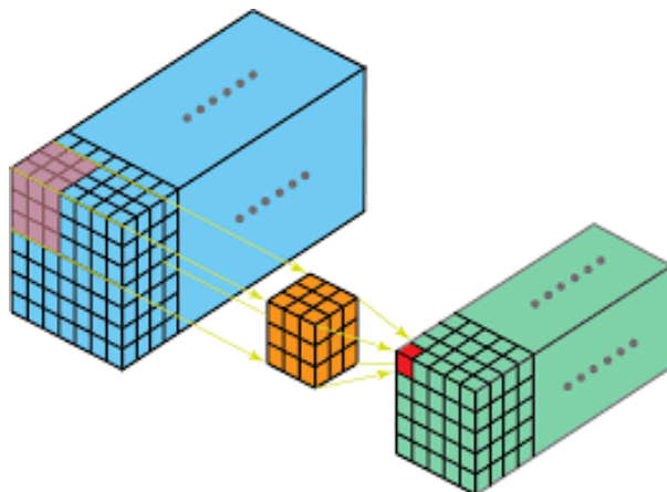
Figure 2: Demonstration of 3D convolution.
